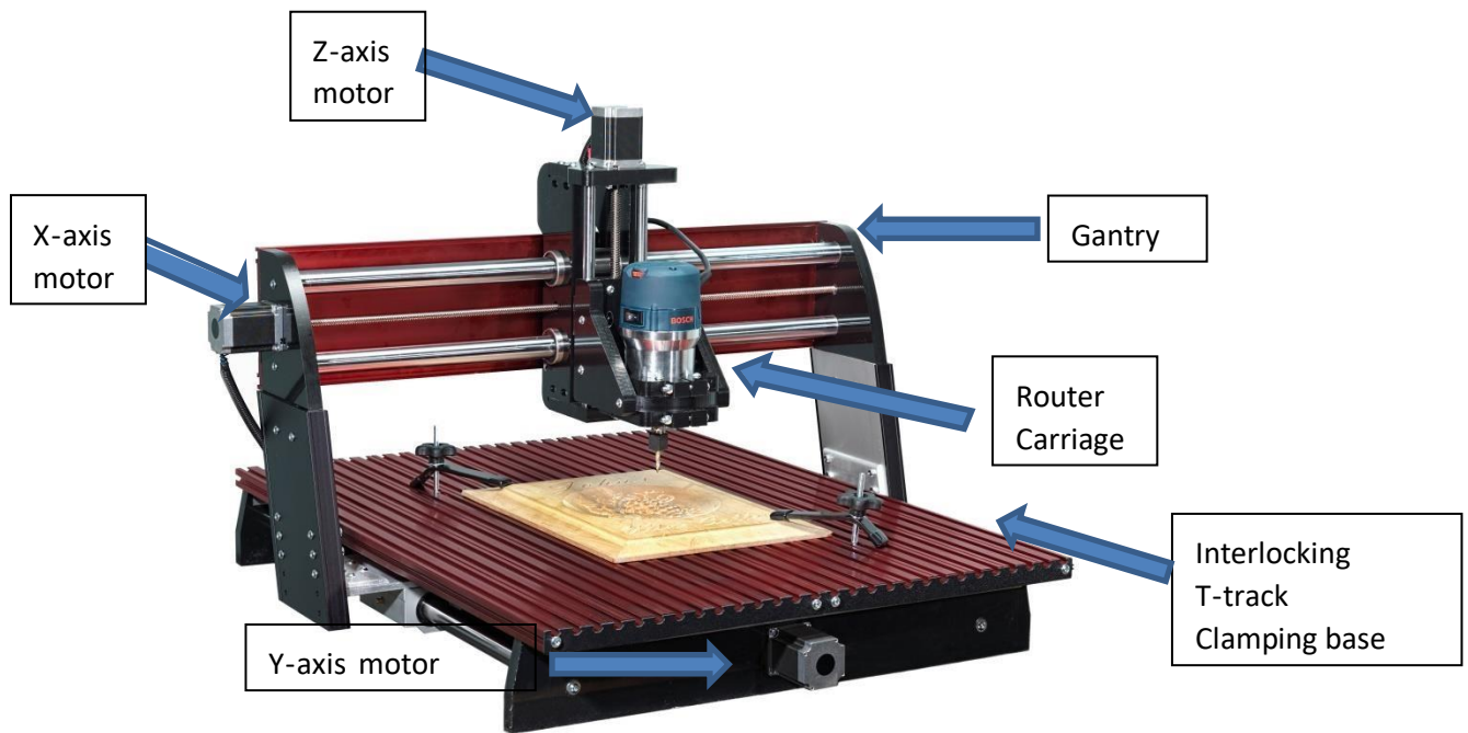
CNC Shark HD4 Core Components
